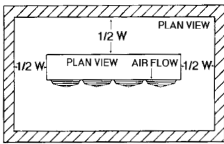
One evaporator
