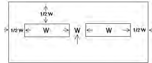
Two evaporators
