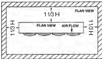
One evaporator
