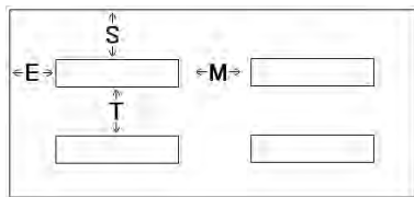
Recommended Maximum - Minimum Dimensions for Center Mount Unit Cooler Installations.
