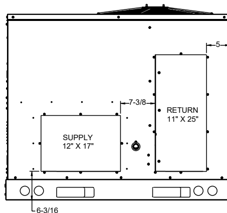
HORIZONTAL DISCHARGE DUCT CONNECTIONS
