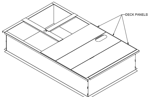
ROOF CURB INSTALLATION
