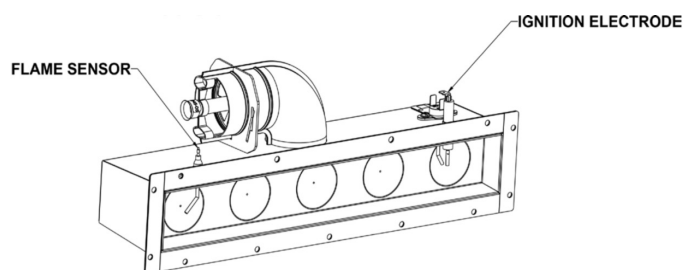
FLAME SENSOR AND IGNITION ELECTRODE LOCATION (ULN ONLY)
