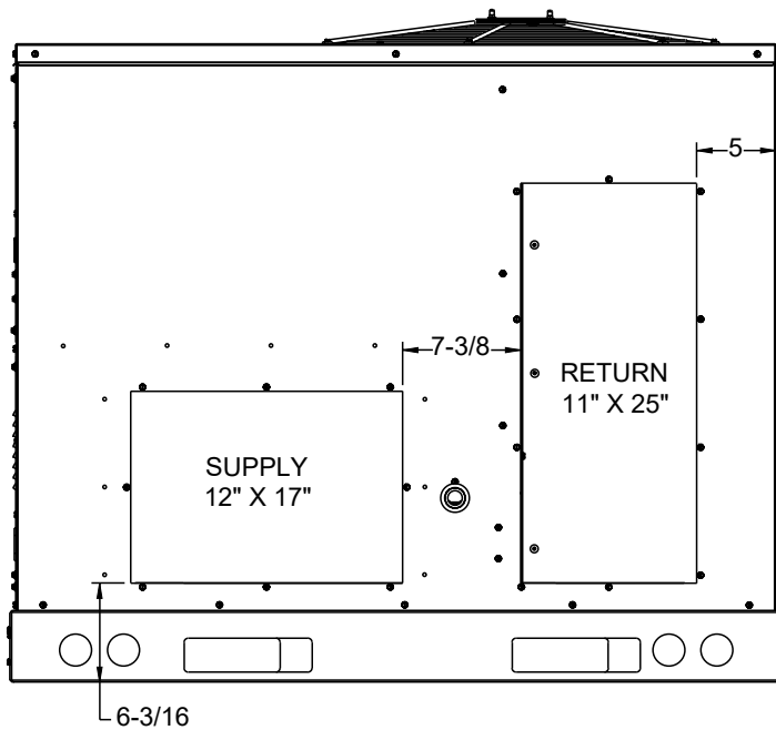
HORIZONTAL DISCHARGE
