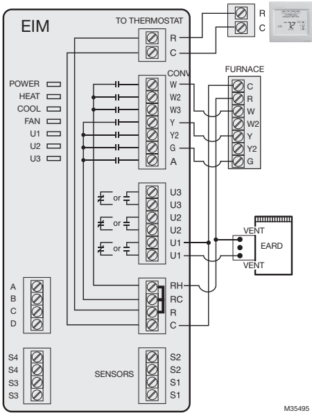
Fig. 3. Wiring an EARD to a VisionPRO® with RedLINK™.
