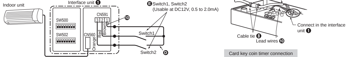
Card key coin timer connection
