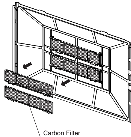
Fig. 17 – Carbon Filter
