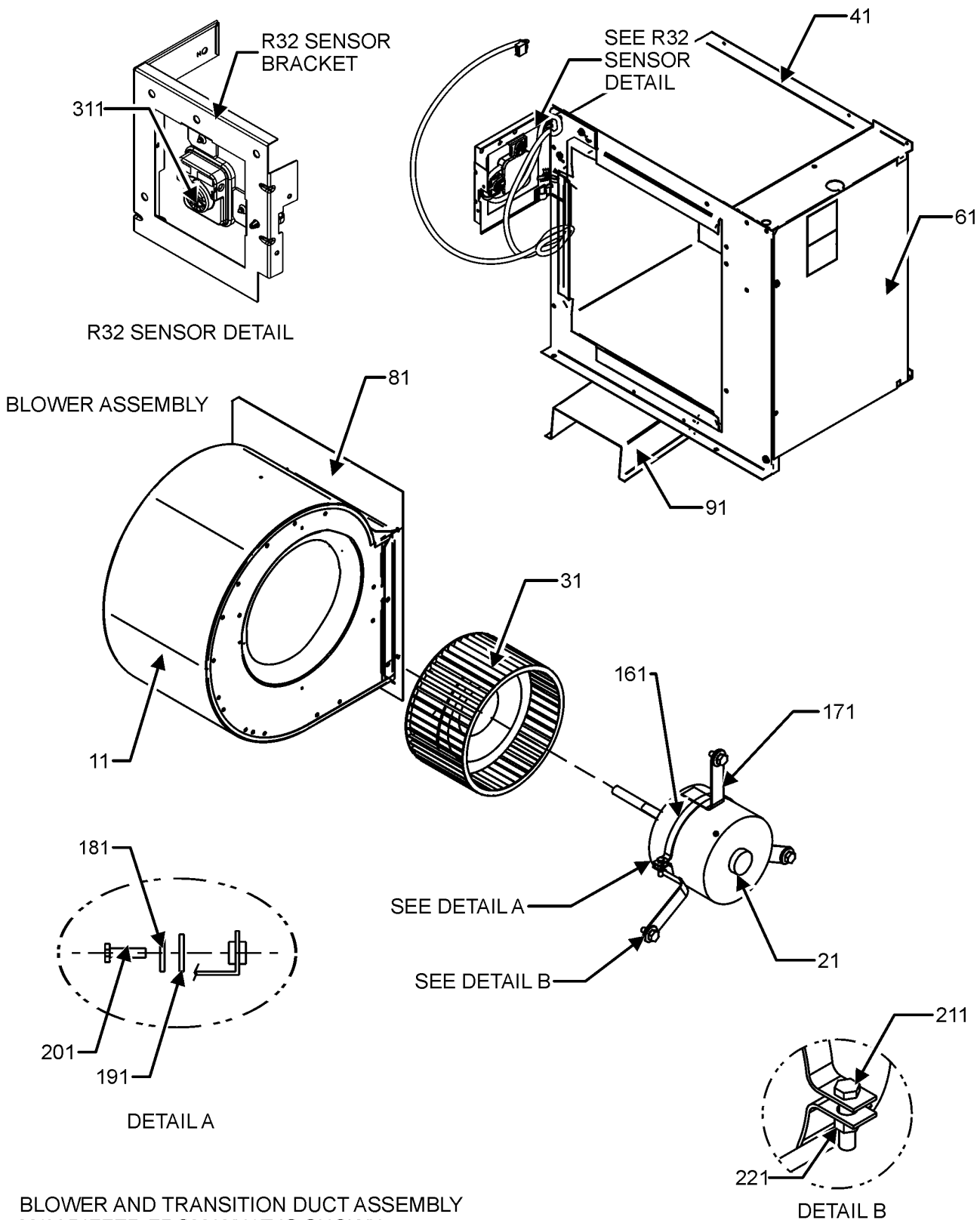
TRANSITION DUCT ASSEMBLY
