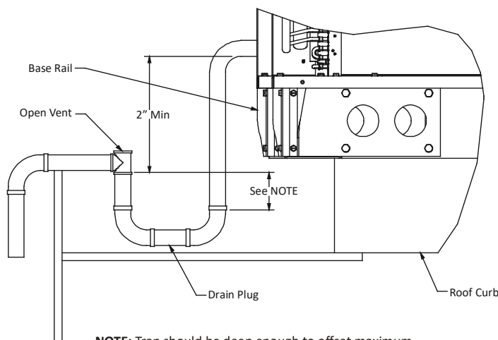
DRAIN CONNECTION FIGURE 12
