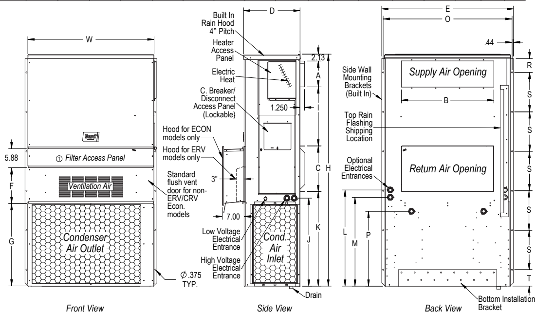
DIMENSIONS OF W18-36L BASIC UNIT FOR ARCHITECTURAL & INSTALLATION REQUIREMENTS (NOMINAL)
