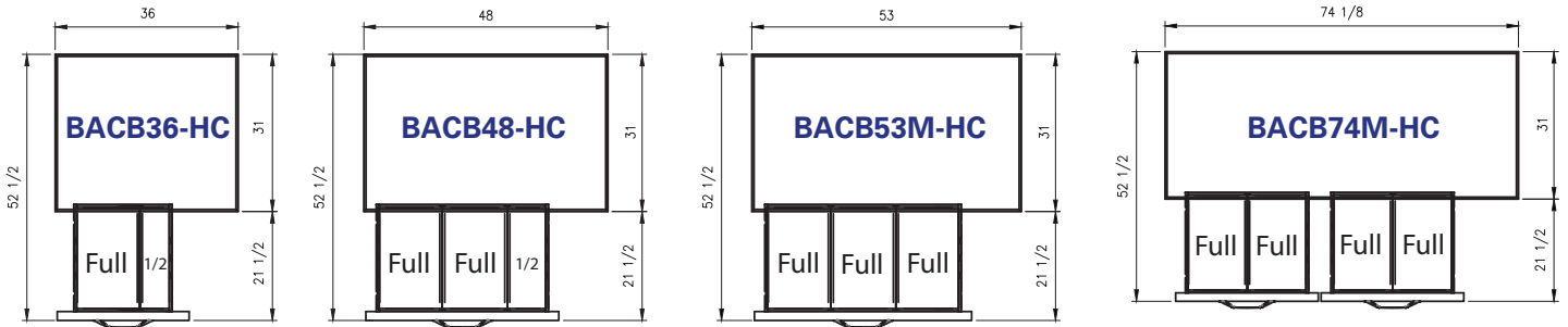
- Front View -
