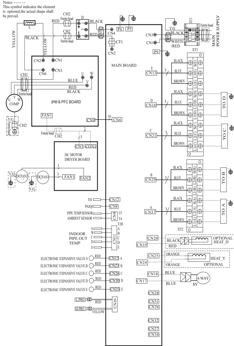
Fig. 13 – Wiring Diagrams 36K – 4 Zone Max
