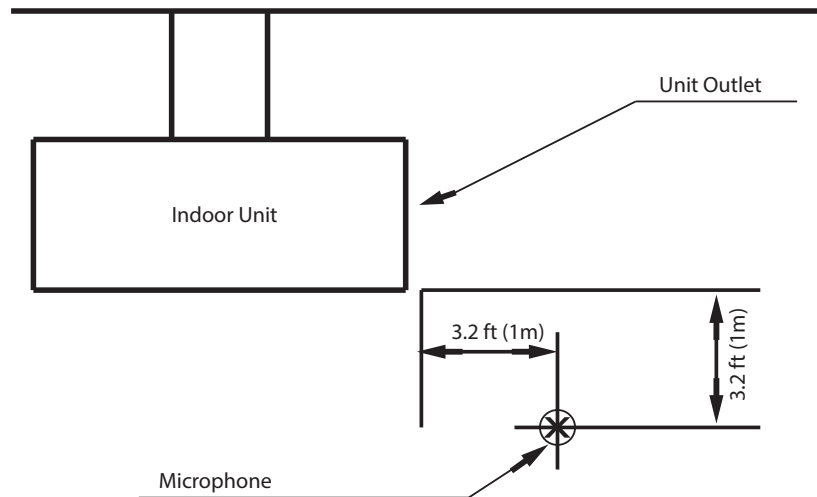
Fig. 6 – Sound Pressure Testing Method
