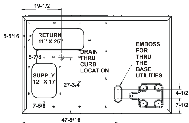
VERTICAL DISCHARGE
