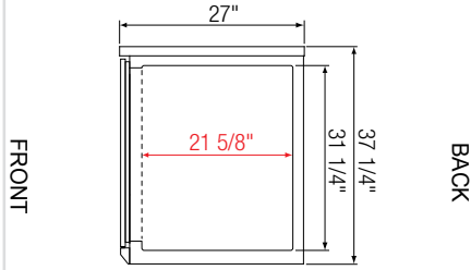
Side View (all models except EBB23G)
