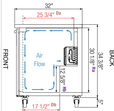
Side View & Air Flow (EBB23G)
