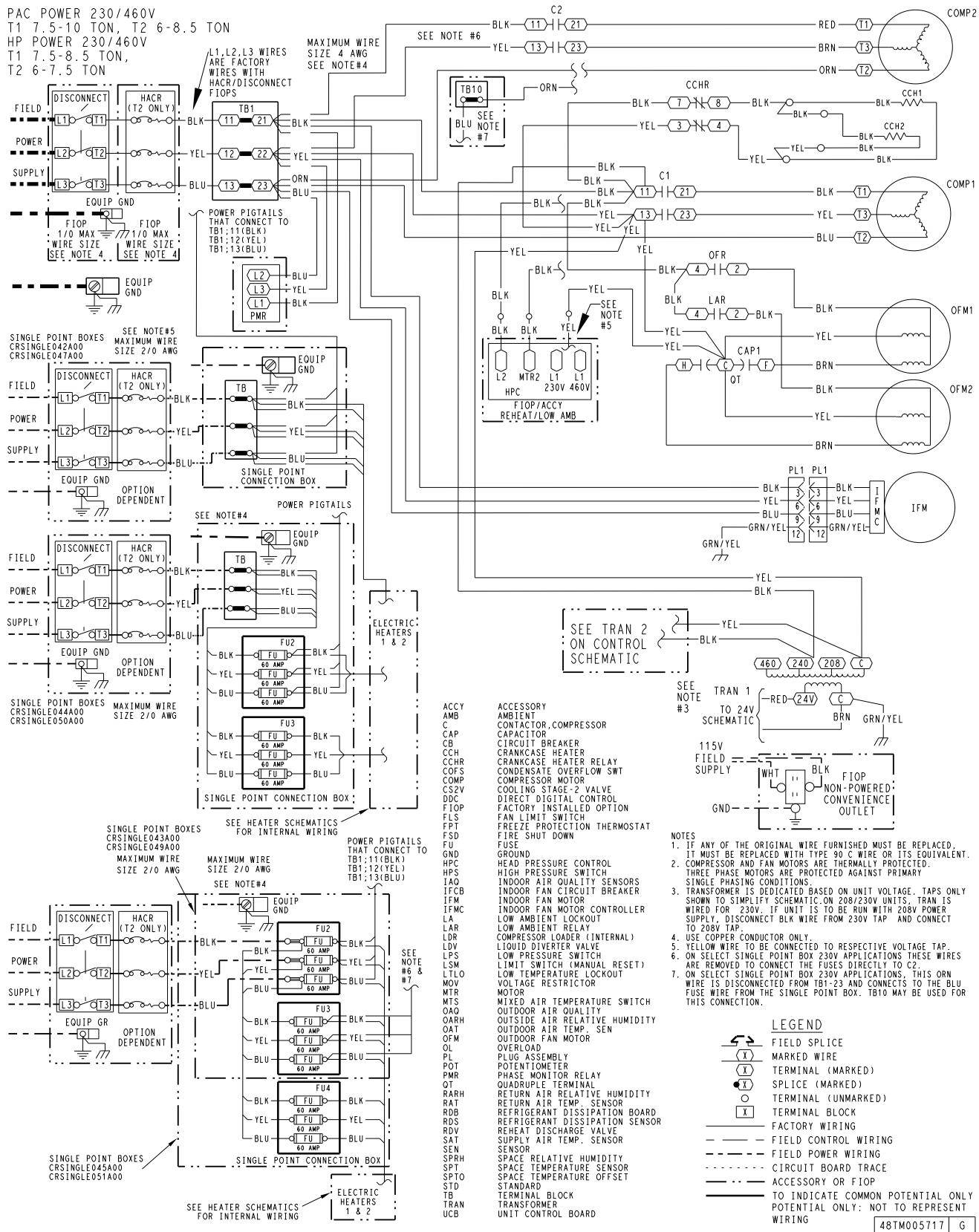
Typical Power Wiring Diagram — RAF090-120 208-230/460-3-60 Unit with Electromechanical Controller
