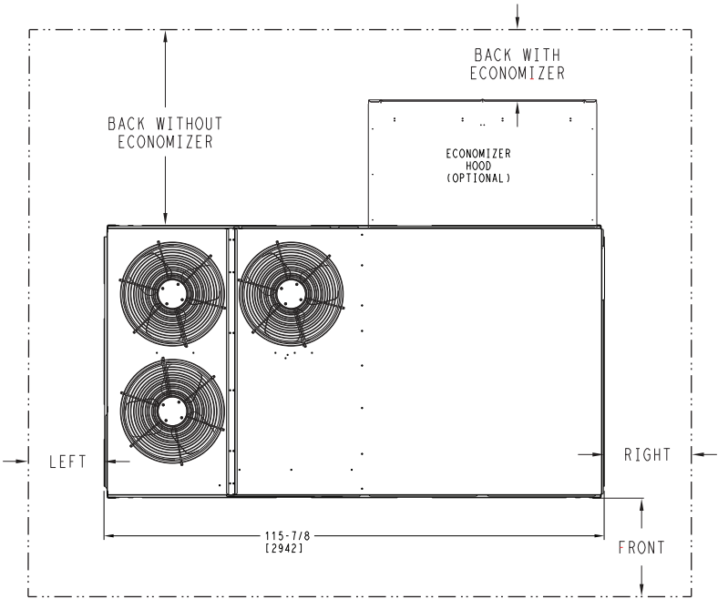
RAF180 Base Unit Dimensions — Clearance
