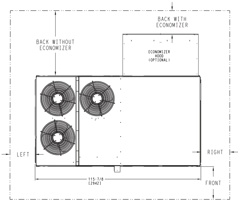
CLEARANCE a,b
