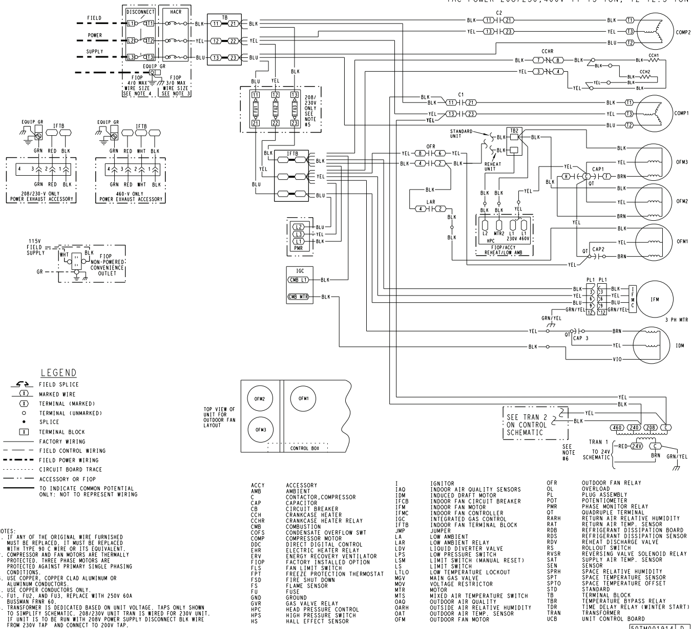
Typical Power Wiring Diagram — RGF180 208-230/460-3-60 Unit with Electromechanical Controller
