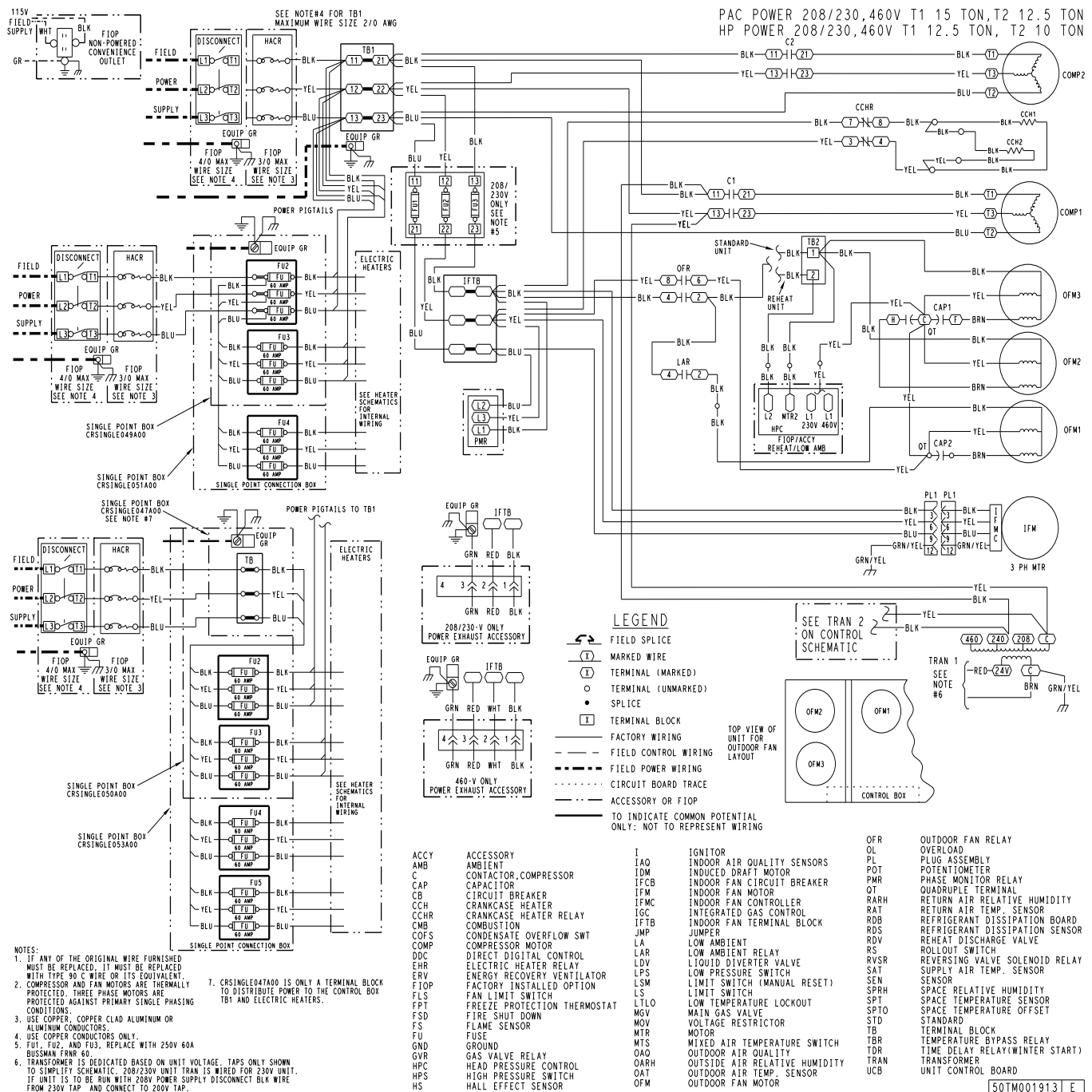
Typical Power Wiring Diagram — RAF180 208-230/460-3-60 Unit with Electromechanical Controller
