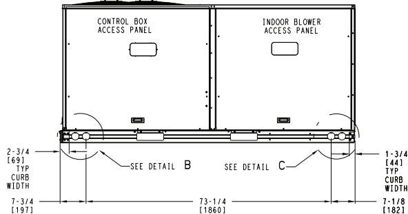
FRONT
