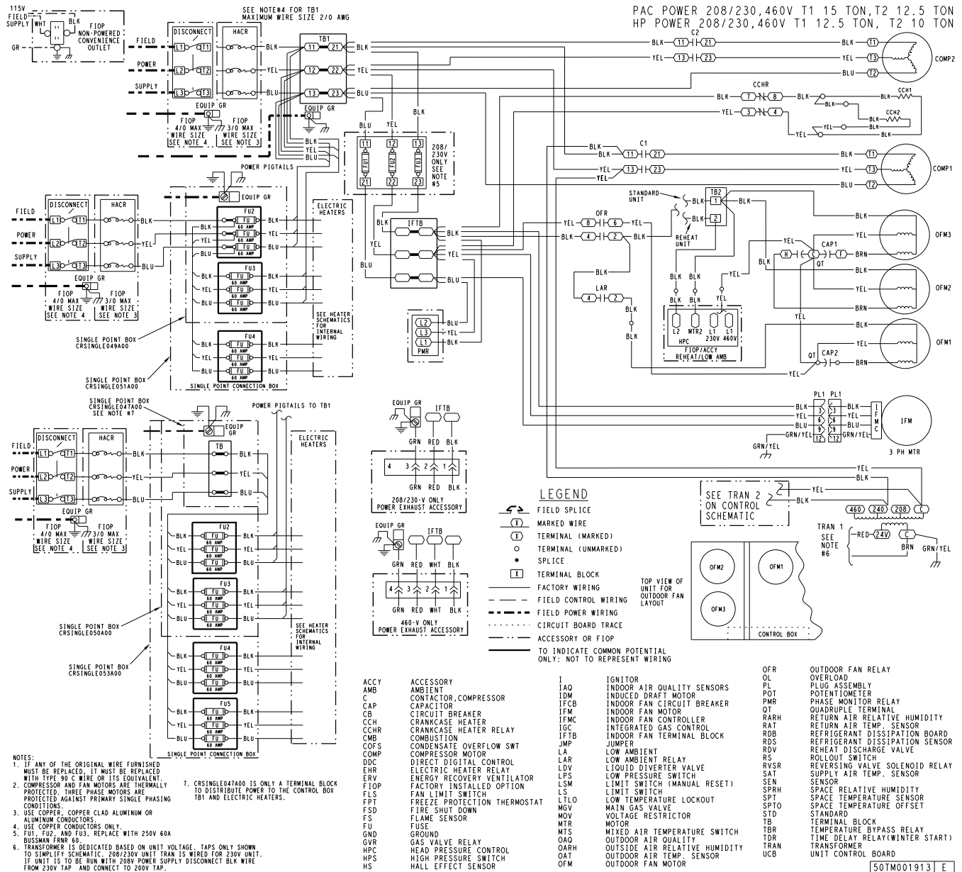
RHF150 Power Wiring Diagram, 208/230, 460-3-60 Shown
