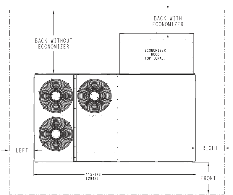
RHF150 Base Unit Dimensions — Clearances
