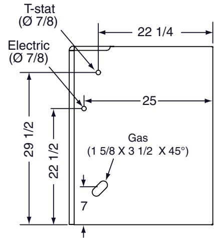
RIGHT SIDE
