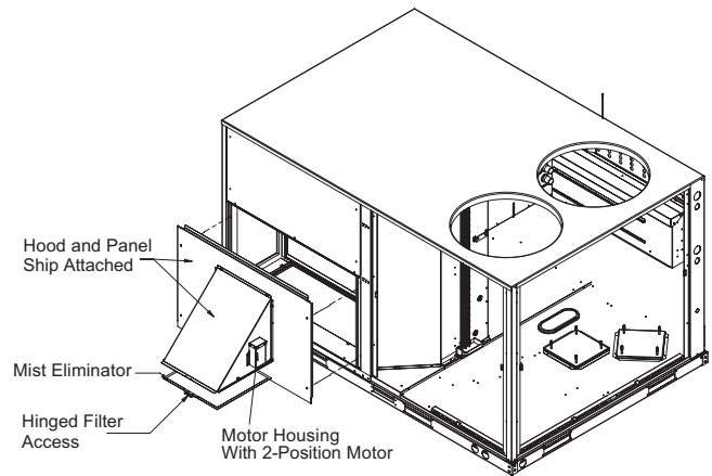
Figure 1. JAYDMPR310* damper assembly
