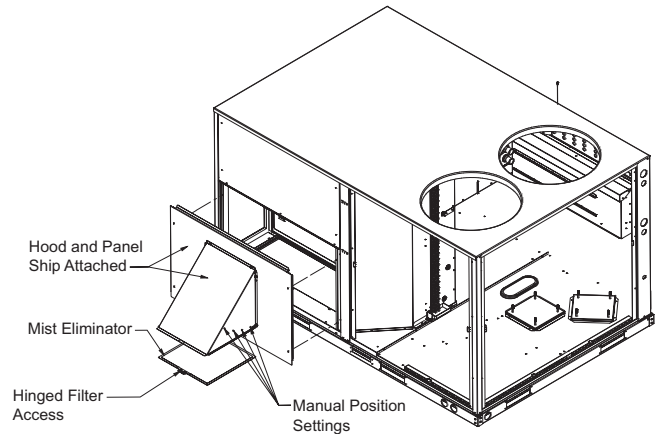
Figure 1. JAYDMPR311* damper assembly
