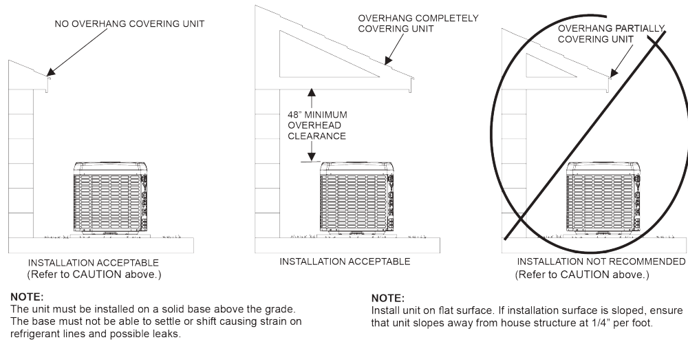
Figure 4: Typical installation
